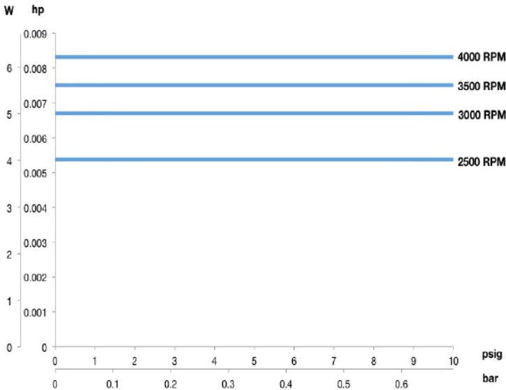
Power Consumption
