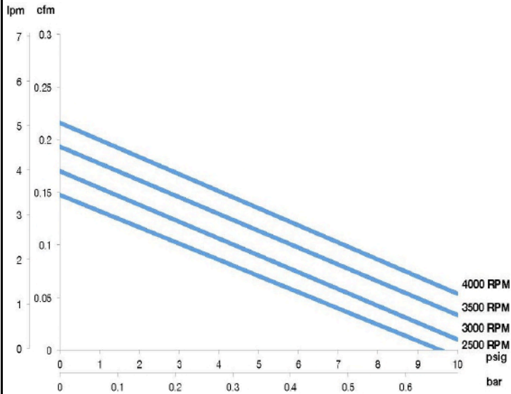
Flow Characteristics
