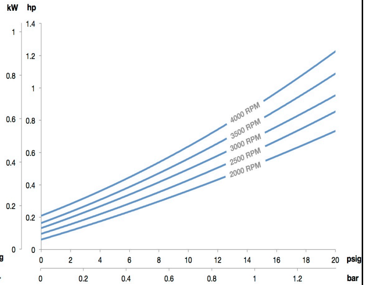
Power Consumption
