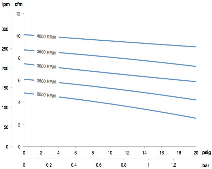
Flow Characteristics
