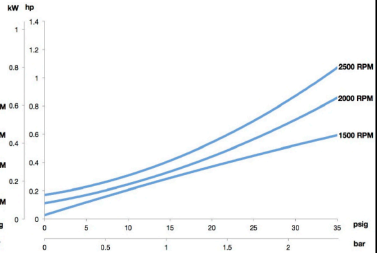
Power Consumption
