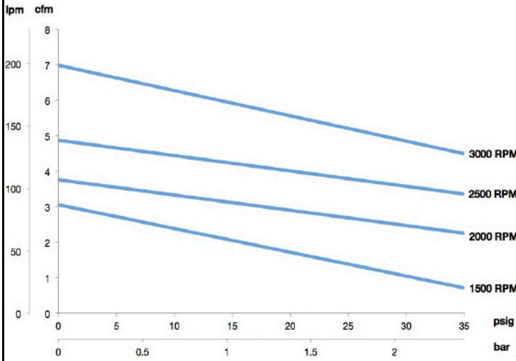
Flow Characteristics
